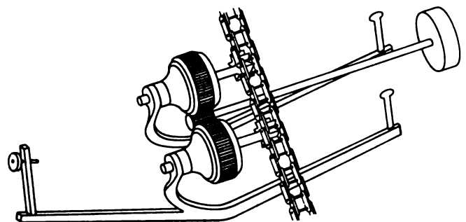
Figure 8-19. Power-actuated setworks.
